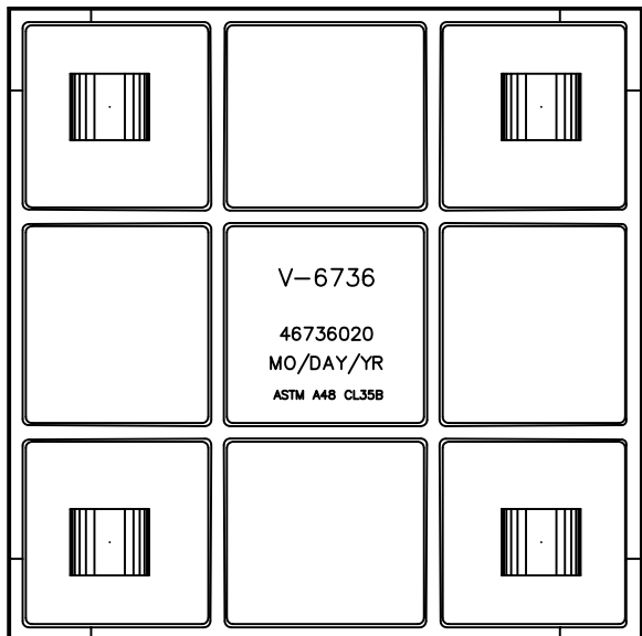
COVER BOTTOM VIEW
