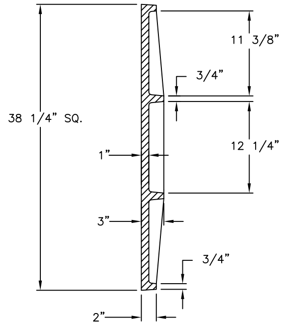
COVER SECTION
