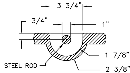
(4) TYPE 4 STEEL PICKBARS PICKBAR DETAIL
